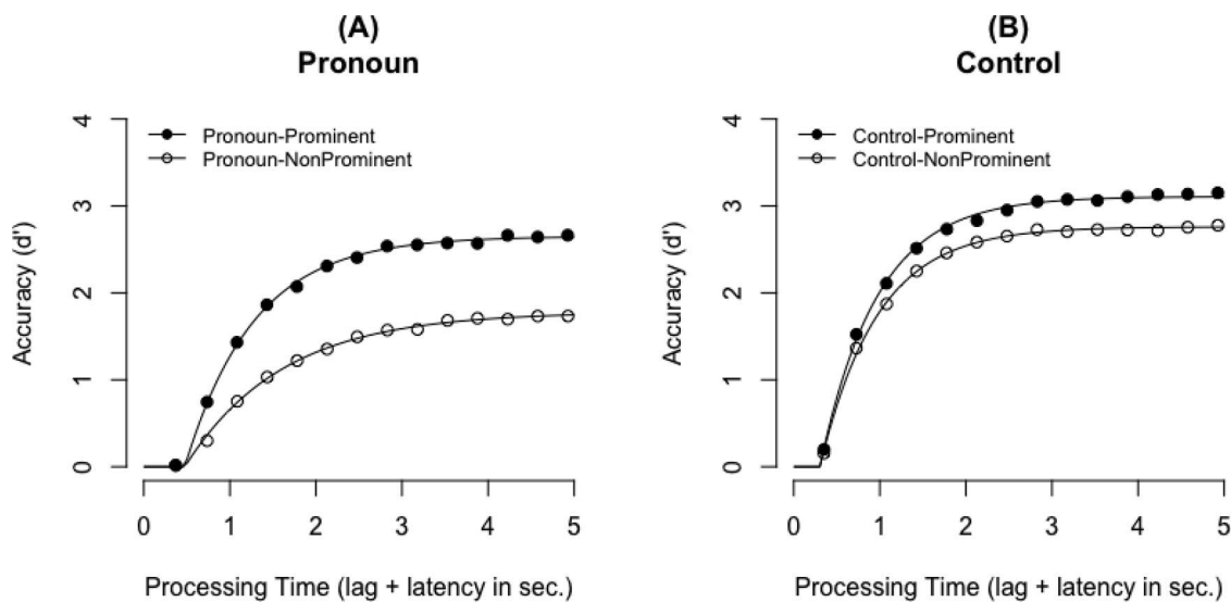
Figure 1. Averaged d' values by condition and response time, as well as the smoothed curves that represent the best fitting model of the average data for the pronoun and control conditions.
