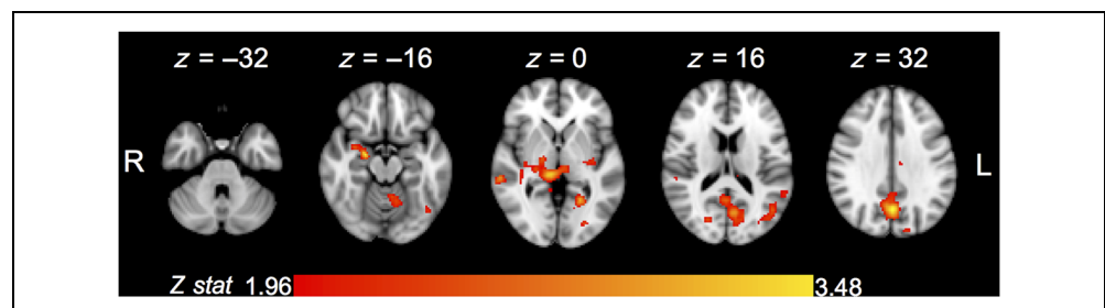
Figure 3. Axial views ( z = -32 mm to z = 32 mm) for the univariate scene-by-scene (item-specific) learning analysis, collapsed across all three exposure runs.
