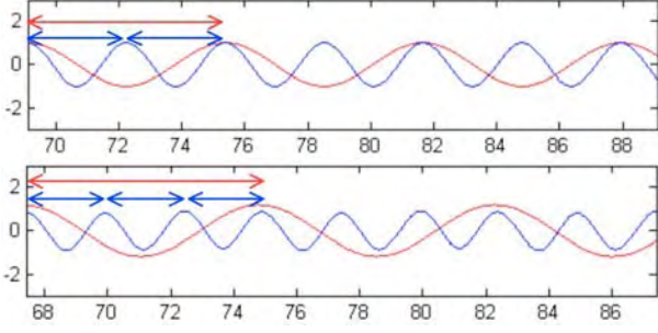
Figure 4: Steady-state waves of foot (slow) and syllable (fast) oscillators (top panel: two syllables per foot; bottom panel: three syllables per foot). Coupling strengths to syllable and foot are 5 and 1, respectively. Vertical axis is oscillator position and horizontal axis is time.
