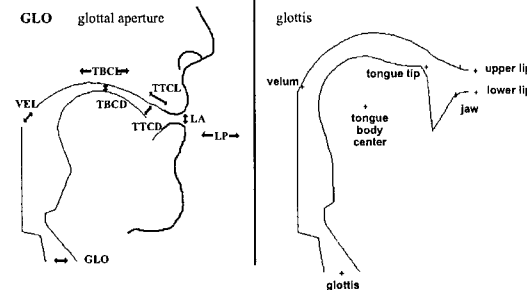
Figure 2: Mapping between tract variables and their involving articulators. Tract variables are defined in constriction degree (LA, TTCD, TBCD, VEL, GLO), and location (LP, TTCL, TBCL) in some cases.
