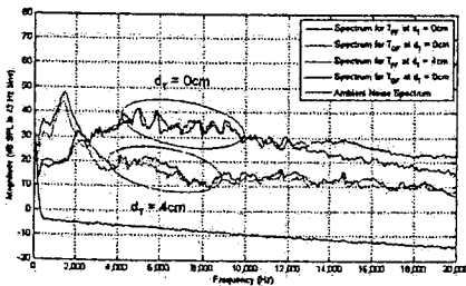
Figure 3: Spectra comparing tongues with flat constriction, and grooved vs. flat inlet, for 0 and 4 cm front cavity length. Flowrate is 40 l/min.
