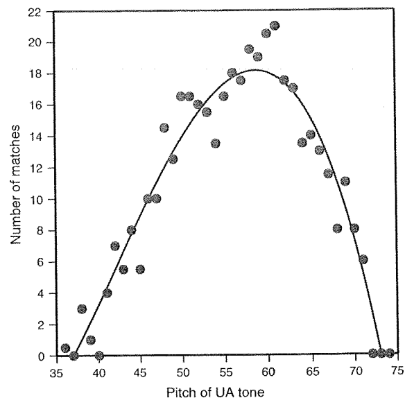
Fig. 5 Experiment 2A: frequency histogram of MIDI pitches of UA tones chosen as matches for OA tones, for all OA tones combined. The function fitted to the data is a cubic polynomial
