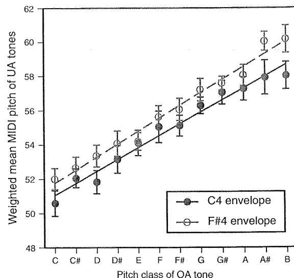
Fig. 7 Experiment 2B: mean subjective pitch heights (weighted mean of MIDI pitches of UA comparison tones) of OA tones with two different spectral envelope centers (C4 and F#4)
