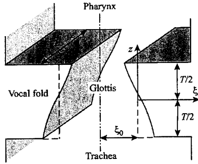
FIG. 1. Vocal-fold model (after Titze, 1988).
