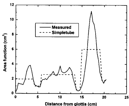
Fig. 4. Measured area function and simple-tube area function.
