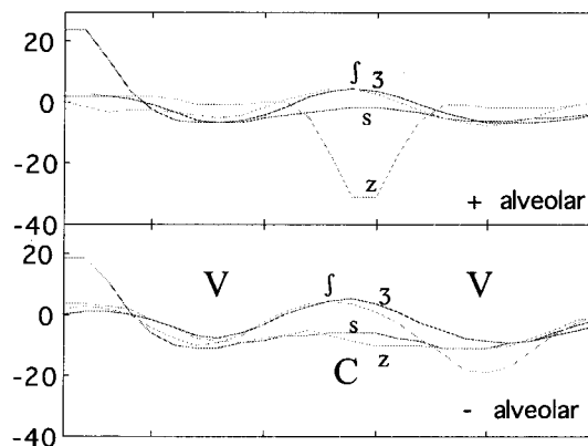
Figure 6: /asa/, /aʃa/, /aza/, /aʒa/. At C, ʃ, ʒ > s > z .
