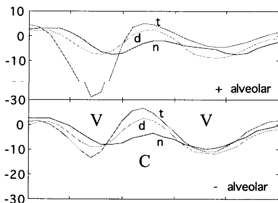
Figure 5: Averaged relative pressure for /ata/, /ada/, /ana/. At offset C, t > d > n .
