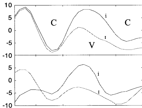
Figure 8: /bib/, /bɪb/. The tense vowel shows higher relative pressure consistent with tongue bracing.
