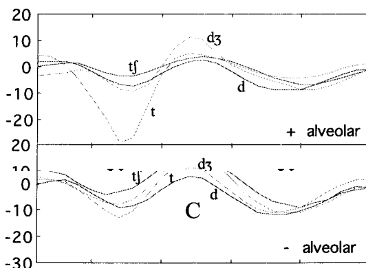
Figure 7: /atʃa/, /adʒa/, /ata/, /ada/. At C, d_3 > t, tʃ > d .
