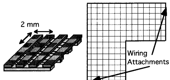
Figure 1: a) Capacitive sheet forms sensels at electrode overlap points; b) Trimmed layout showing approximate locations of potentially addressable sensels
