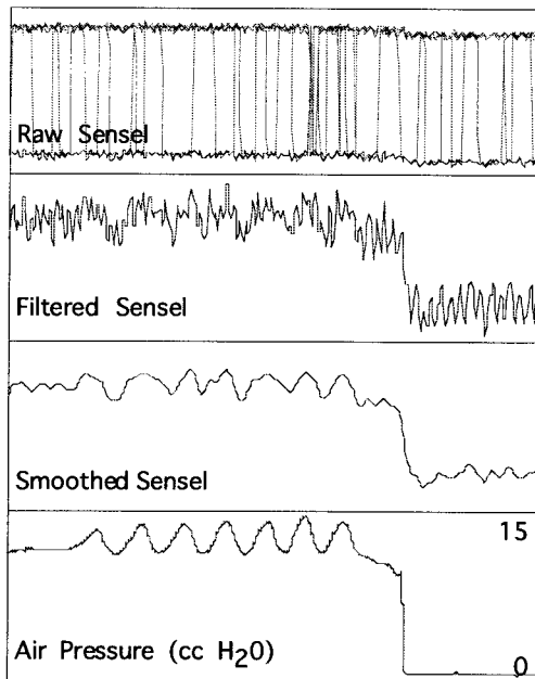
Figure 2: Sample balloon calibration data for one sensel. Smoothed data tracks pressure with reasonable fidelity.
