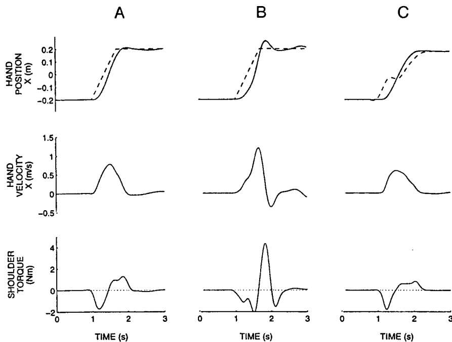
FIG. 7. Effects of the shape of the equilibrium shift and the model of force generation on simulated multijoint movements. A : simulated movements that result when a constant-rate equilibrium shift is used with the model proposed in this paper. B : a constant-rate equilibrium shift was used with the force-generation model proposed by Gomi and Kawato (1996). Net deceleration torques are generated only when the limb position crosses the equilibrium (in this case, after the end of the equilibrium shift). C : to produce smooth movements comparable with that shown in A using the force-generation mechanism proposed by Gomi and Kawato, a nonmonotonic equilibrium shift is required.
