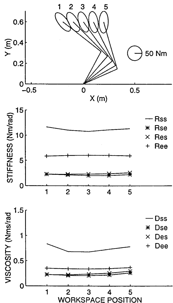
FIG. A1. Simulated hand-stiffness ellipses and joint-stiffness and viscosity matrices for the arm model for 5 static postures.
