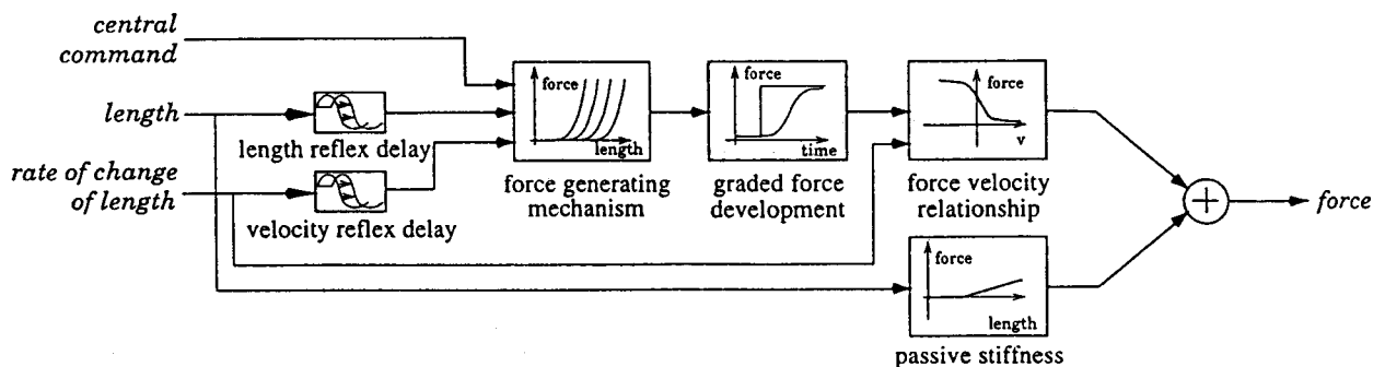
FIG. 1. Schematic representation of the muscle model. Model includes the dependence of force on muscle length and velocity, graded force development over time, passive elastic stiffness, and length and velocity dependent afferent input.
