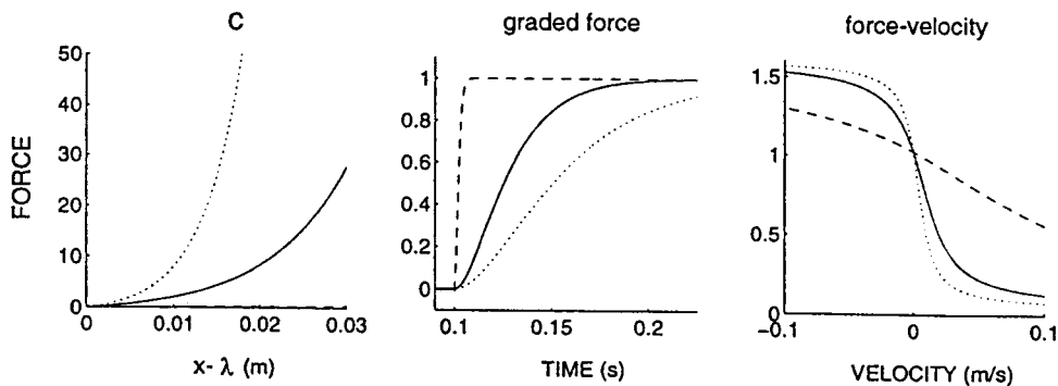
FIG. C1. Range of parameter variation in sensitivity analyses for c (force-length relation), \tau (graded force development), and f_i (force velocity). Vertical axes indicate force (N) for the force-length relation and normalized force for graded force development and the force-velocity relation. Minimum (---), center (—), and maximum (···) levels are indicated for each parameter. Values of c from left to right are 10, 112, and 220 mm -1 . Values of \tau from left to right are 1, 15, and 30 ms. Values of f_i from shallow to steep are 10, 58, and 120 s/m. ( c = 112 mm -1 , \tau = 15 ms, and f_i = 58 s/m are used for the simulations reported in the main body of the paper.) For force velocity, negative velocities correspond to muscle lengthening and positive values represent muscle shortening.
