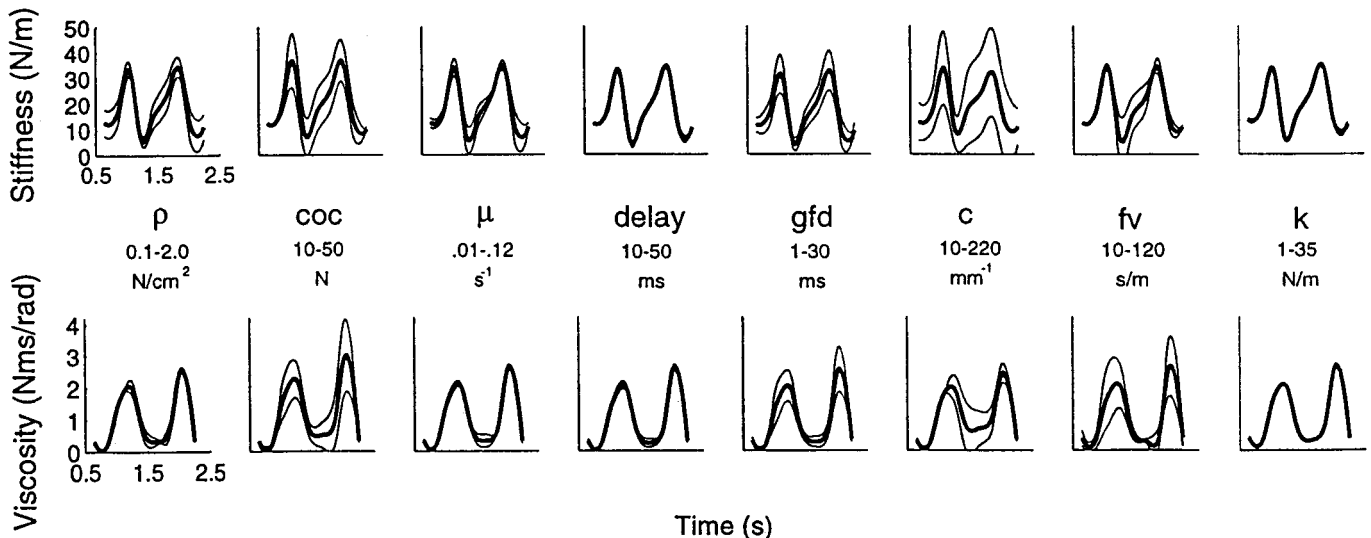
FIG. C3. Estimates of simulated stiffness ( R_{ss} ) and viscosity ( D_{ss} ) during movement resulting from changes in individual model parameters. Means (bold) \pm 1 SD are shown. Abbreviations as in Fig. C2. Numerical estimates of the sensitivity of all 4 terms in the stiffness and viscosity matrices to model parameter change are given in Fig. C4.
