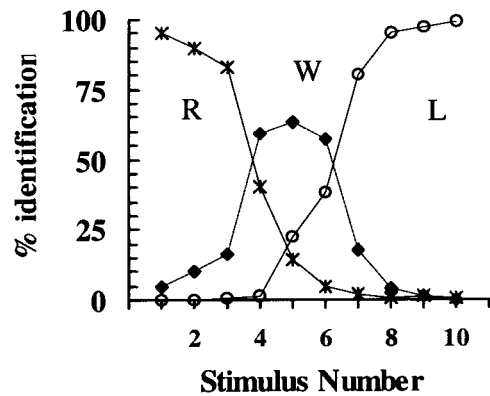
Figure 3. Identification data in Experiment 2 (10 subjects)
