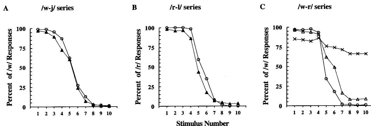
Figure 1. Identification data for French (triangles or x for "W-dominant") in this study, and for Americans (circles) in [2].
