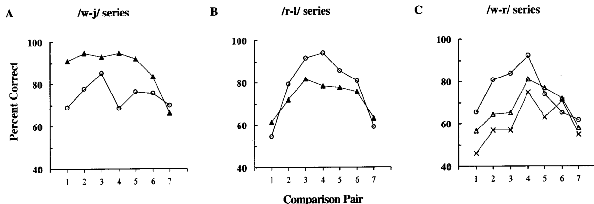
Figure 2. Discrimination data for French (triangles or x for "W-dominant") in this study, and for Americans (circles) in [2].
