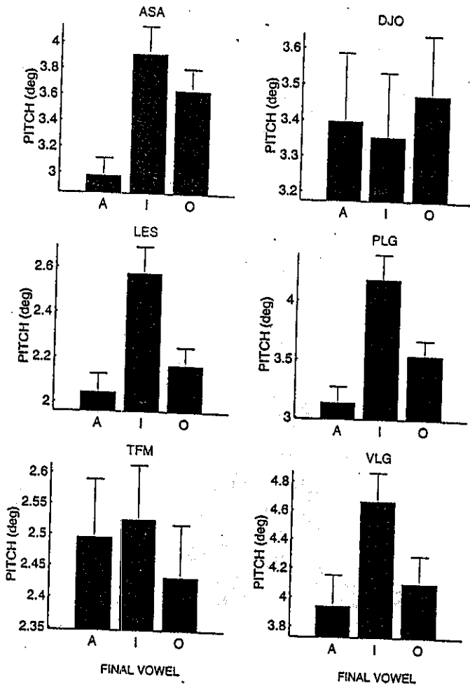
Figure 7. Mean pitch amplitude during jaw-closing movements for different final vowels in VCV utterances (SEs are shown).
