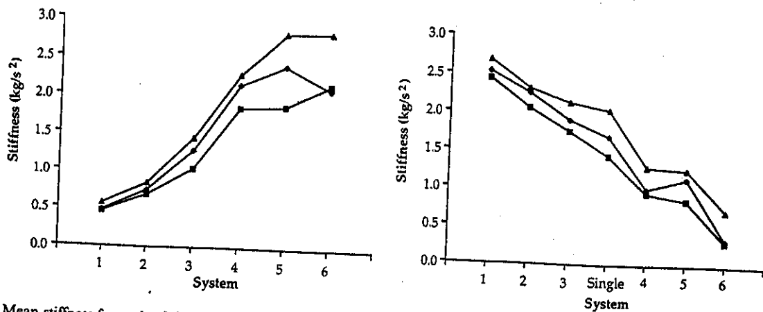
Figure 4. Mean stiffness for each of six different wrist-pendulum systems at three different levels of ankle torque: Means of the data from 3 participants. (The left- and right-hand panels contain data from the left and right hands, respectively. Squares represent 0% torque; diamonds, 25% torque; triangles, 50% torque.)
