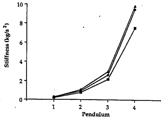
Figure 2. Mean stiffness values for each of four different pendulums at three different levels of torque exerted at the opposite hand. (Derived from data reported by Kugler & Turvey [1987]. Squares represent 0% torque; diamonds, 25% torque; triangles, 50% torque.)
