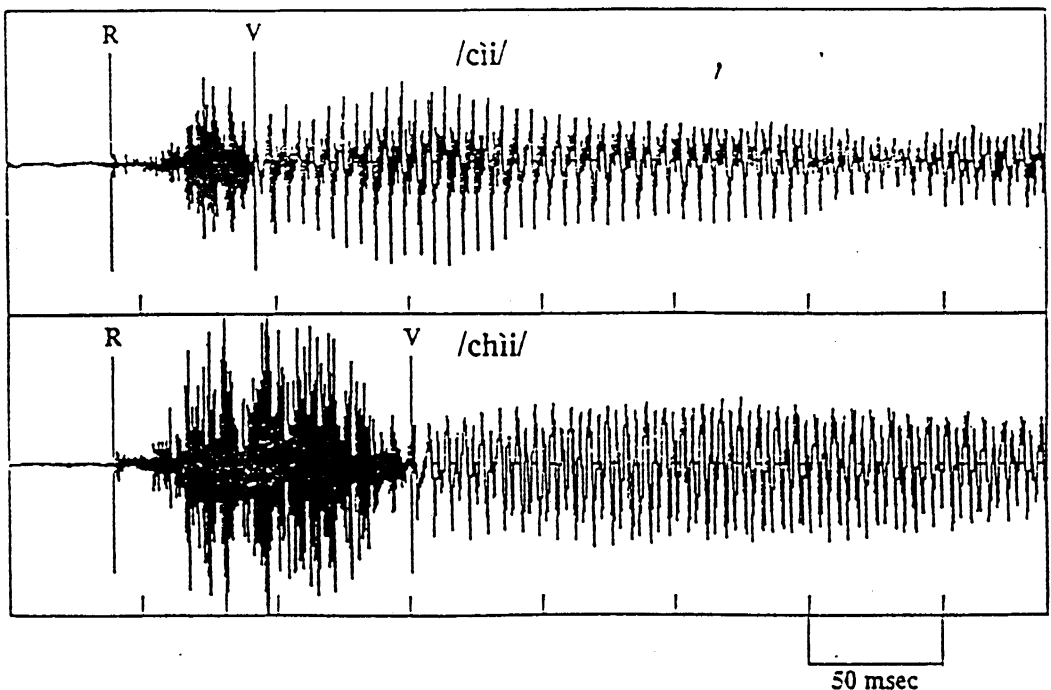
Figure 2 Waveforms showing VOT differences in Thai palatal affricates. R - release of oral closure. V - onset of voicing (glottal pulsing). R-V is also the duration of the frication.
