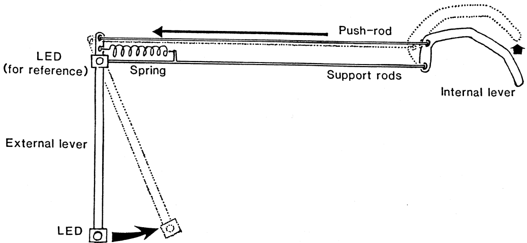
FIGURE 1 Schematic diagram of the Velotrace.
