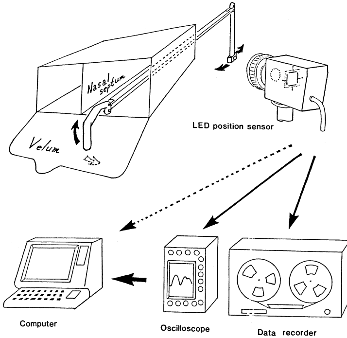
FIGURE 3 Schematic diagram of the recording and processing system.
