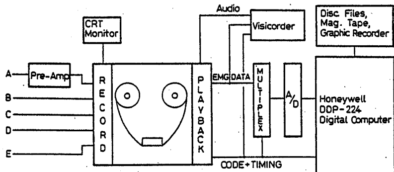
Fig. 1. Blockdiagram of the EMG data acquisition and processing system. A = EMG (8 channels), B = air pressure (2), C = voice, D = banter, E = digital code and timing.
