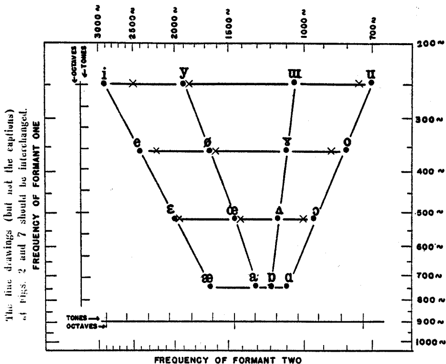
FIG. 2. The acoustic locations of the synthetic vowels, plotted according to the frequency positions of the first and second formants. To make this acoustic plot resemble more closely the familiar vowel quadrilateral (whose coordinates have an articulatory reference), we have reversed the usual order of the frequency scales on both the vertical and horizontal axes and have made the frequency scales logarithmic. (For a detailed comparison of articulatory and acoustic vowel charts see: Martin Joos, op. cit. , pp. 49-59.)
